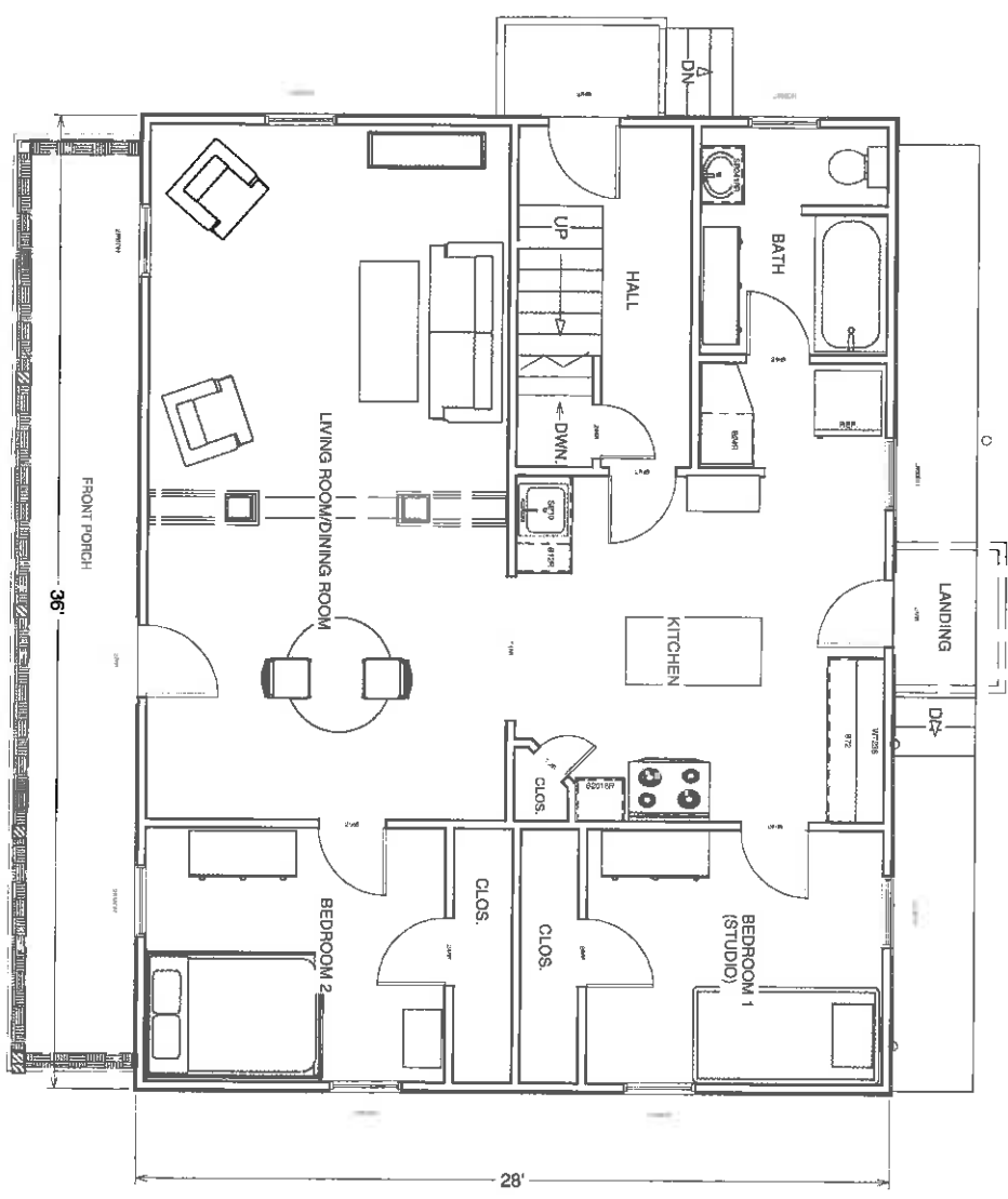
PLAN VIEW/ 2ND FLOOR APARTMENT
